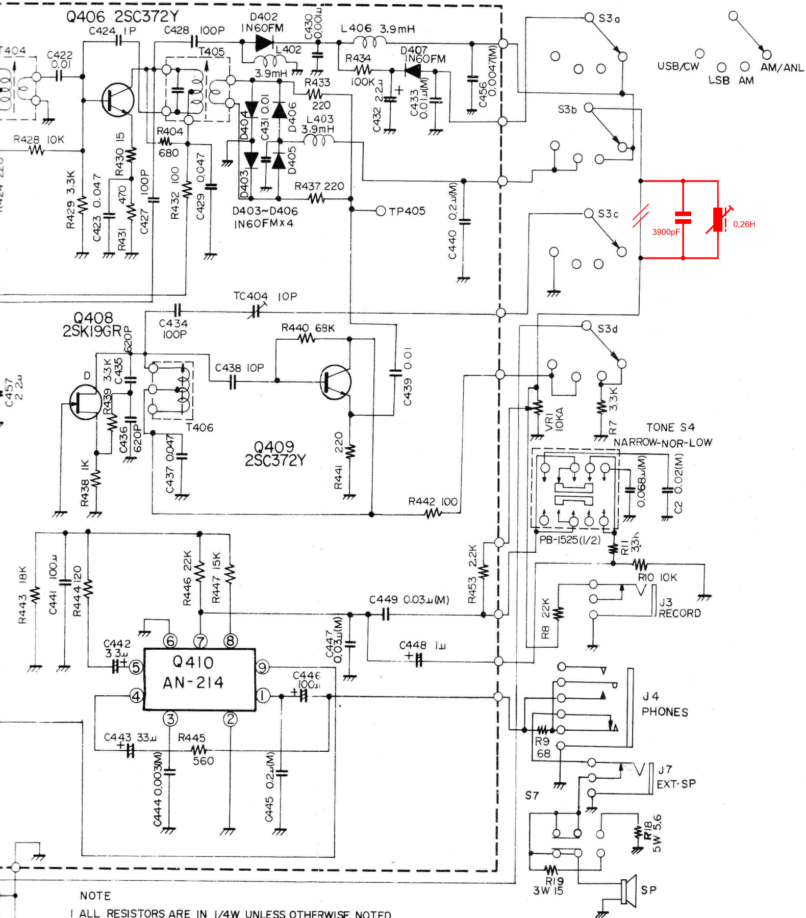
FRG-7 CIRCUIT DIAGRAM
